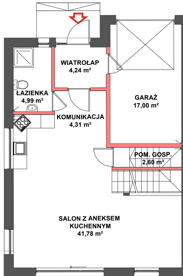
PARTER - 74,92 m 2
